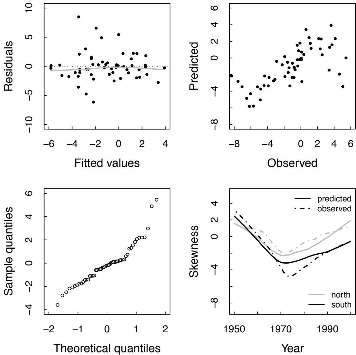
Figure A2. Evaluation plots for the linear skewness model. Shown are the model residuals versus fitted values (top left), the QQ plot of the sample vs theoretical quantiles (bottom left), the predicted versus observed values (top right), and the smoothed time series of predicted and estimated skewness (bottom right) for the north (grey) and south (black) basins.
